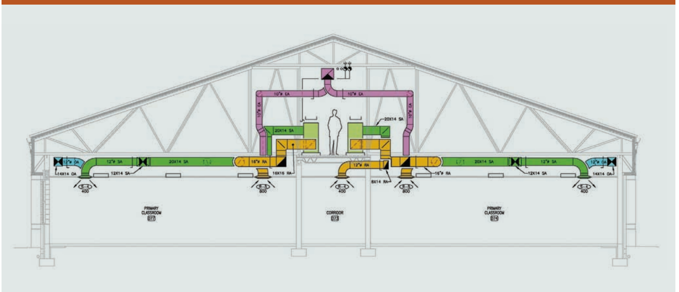
FIGURE 1 TYPICAL CLASSROOM SECTION
